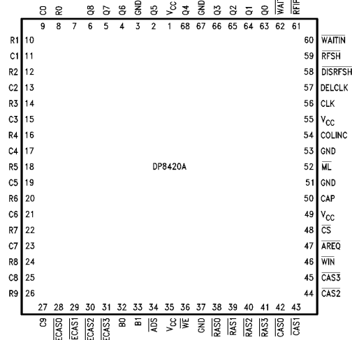
Top View FIGURE 2
